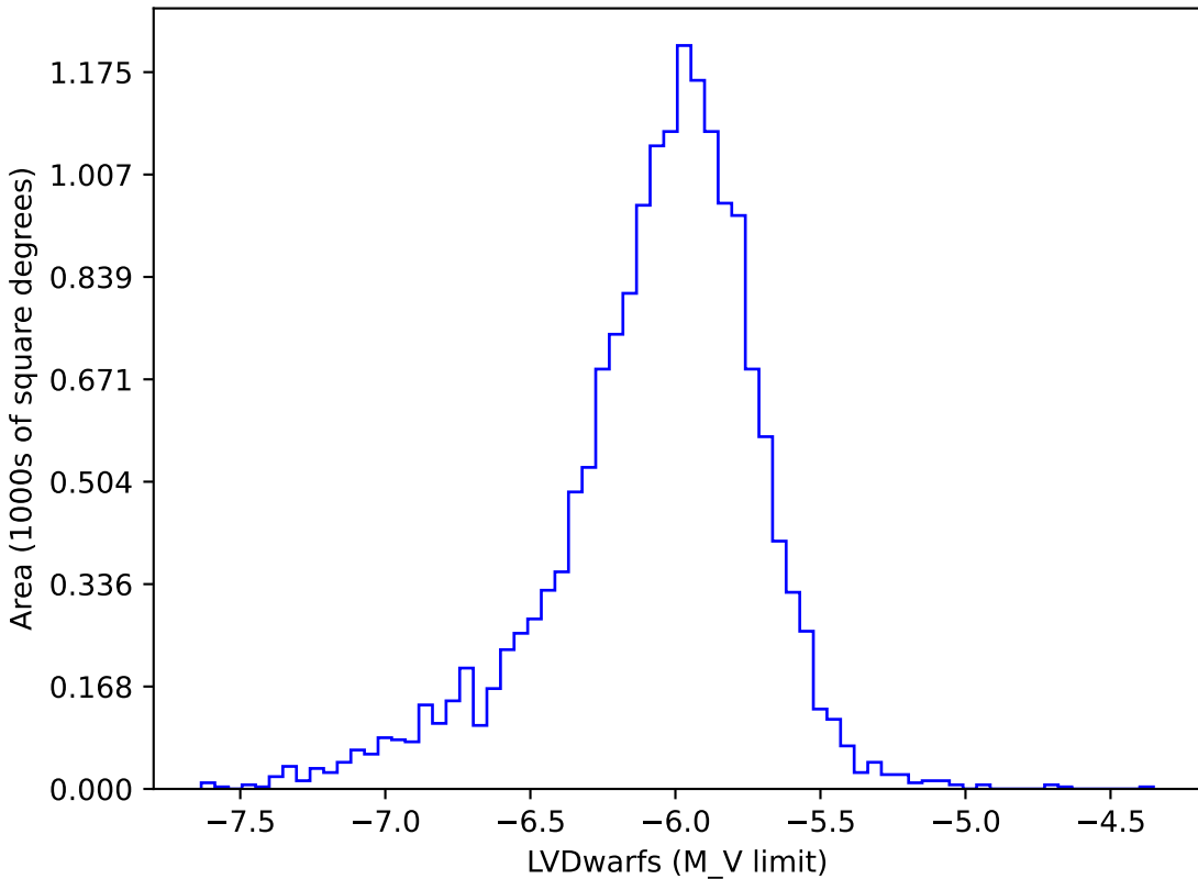
weather_cloudso4v3.5_10yrs gi: LVDwarfs
