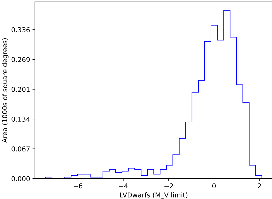
weather_cloudso4v3.5_10yrs gi SCP: LVDwarfs
