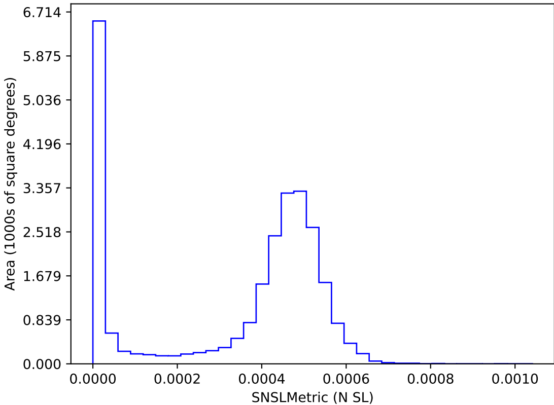
weather_cloudso4v3.5_10yrs : SNSLMetric
