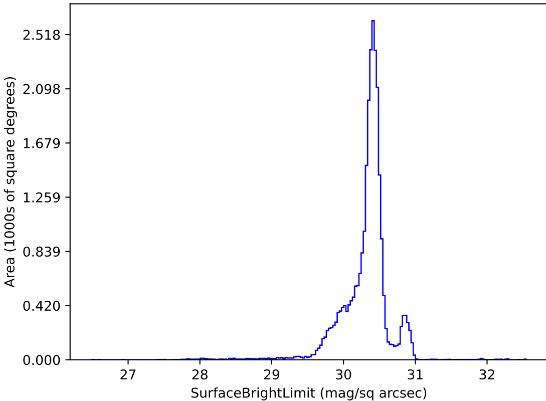
weather_cloudso4v3.5_10yrs g: SurfaceBrightLimit
