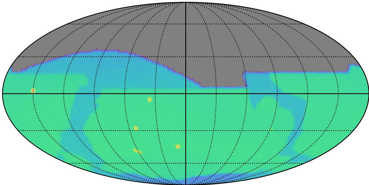
weather_cloudso4v3.5_10yrs r: SurfaceBrightLimit
