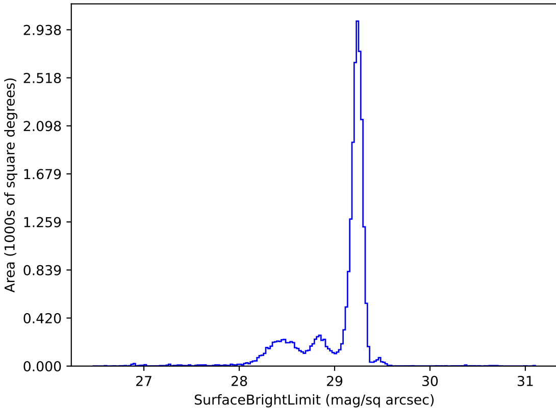
weather_cloudso4v3.5_10yrs u: SurfaceBrightLimit
