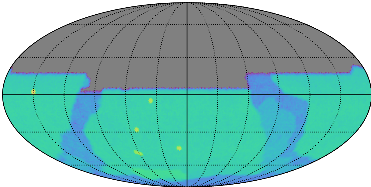
weather_cloudso4v3.5_10yrs u: SurfaceBrightLimit
