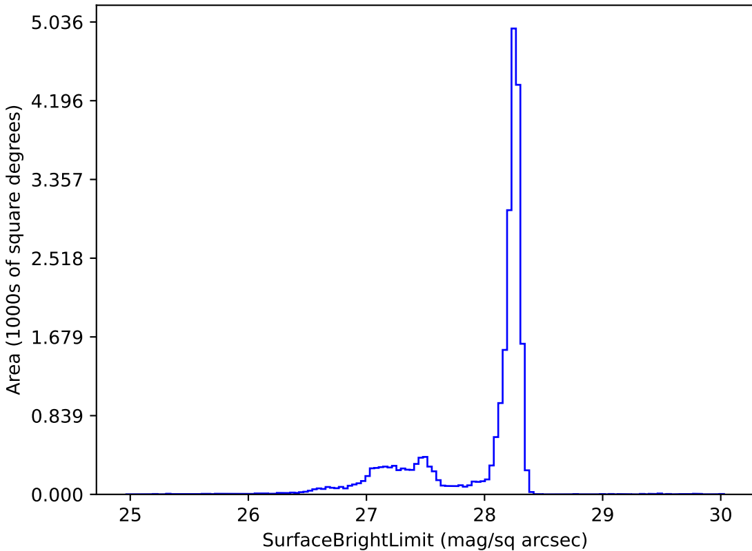
weather_cloudso4v3.5_10yrs y: SurfaceBrightLimit
