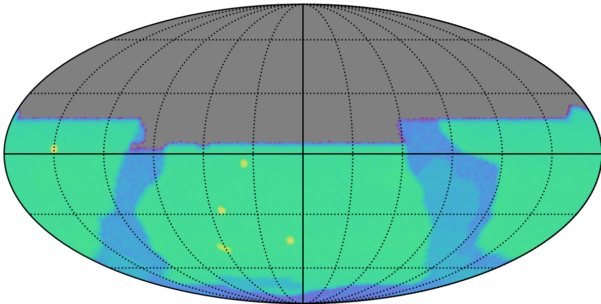
weather_cloudso4v3.5_10yrs y: SurfaceBrightLimit
