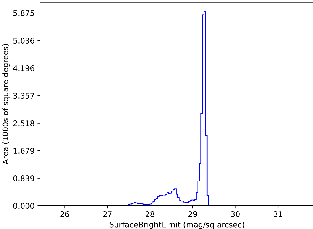
weather_cloudso4v3.5_10yrs z: SurfaceBrightLimit
