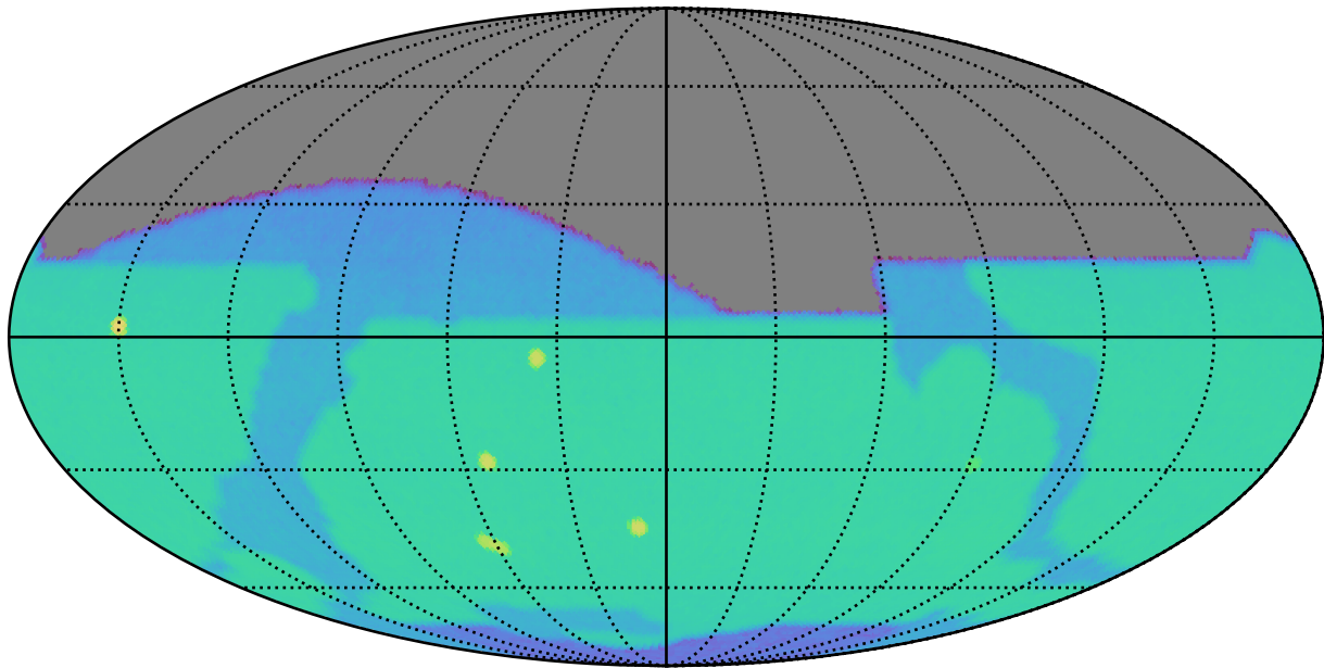
weather_cloudso4v3.5_10yrs z: SurfaceBrightLimit
