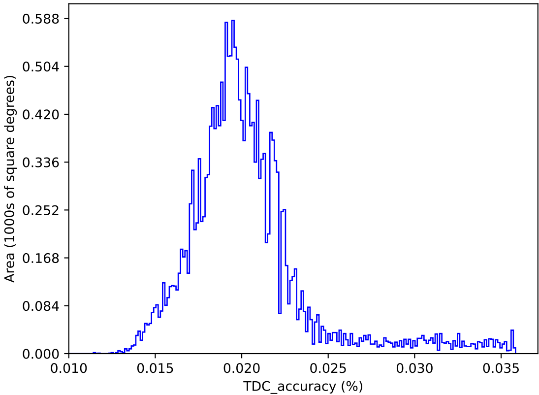
weather_cloudso4v3.5_10yrs : TDC_accuracy
