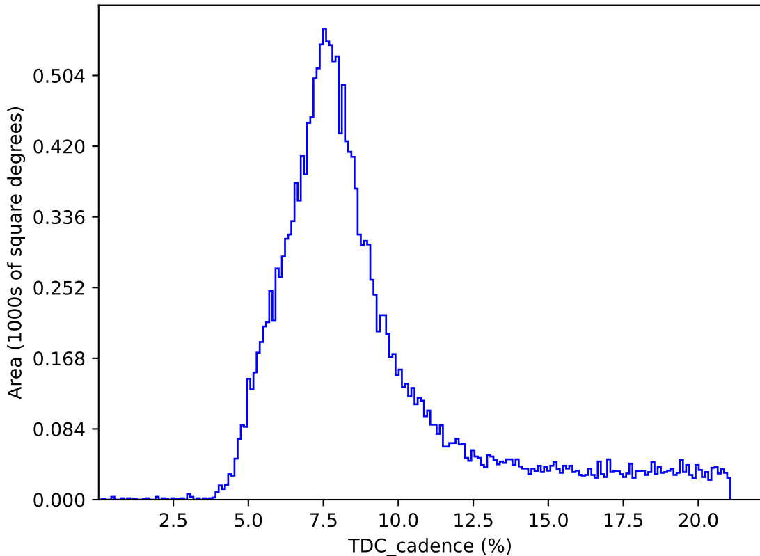
weather_cloudso4v3.5_10yrs : TDC_cadence
