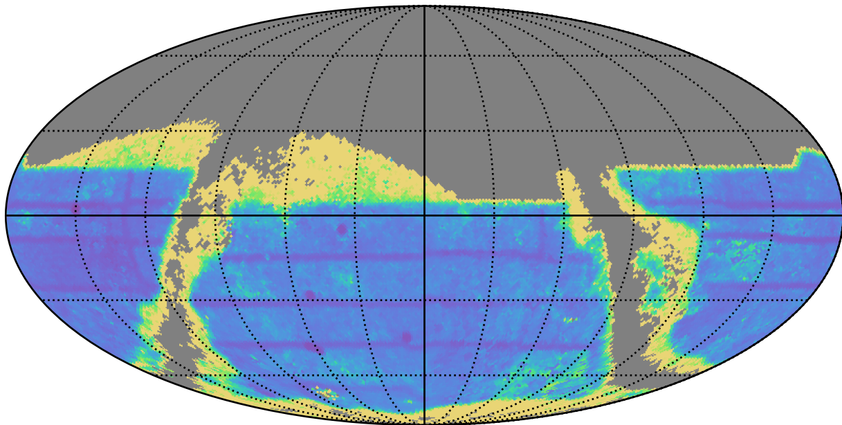
weather_cloudso4v3.5_10yrs : TDC_precision
