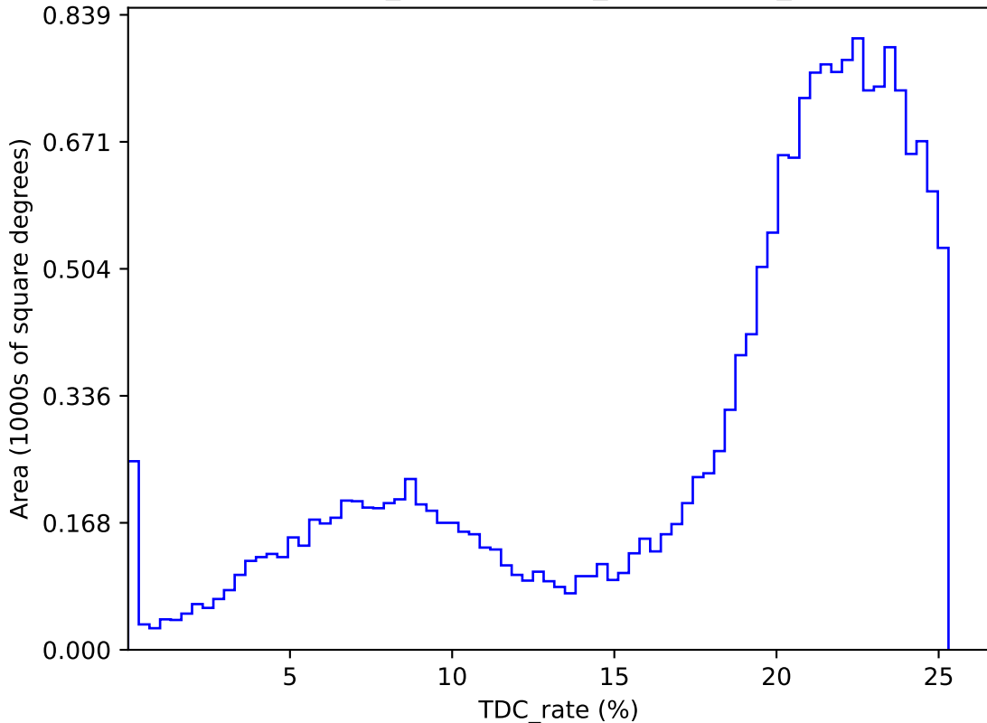
weather_cloudso4v3.5_10yrs : TDC_rate
