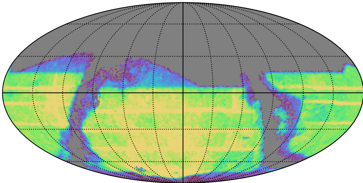
weather_cloudso4v3.5_10yrs : TDC_rate
