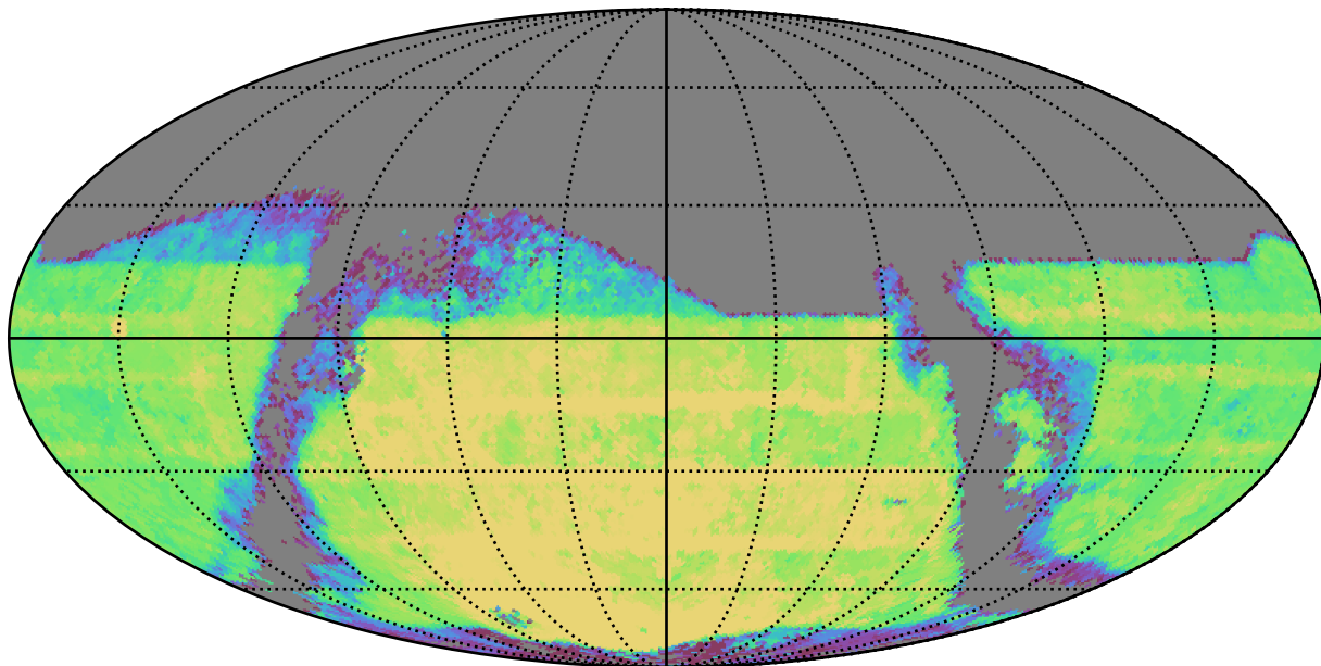
weather_cloudso4v3.5_10yrs : TDC_season
