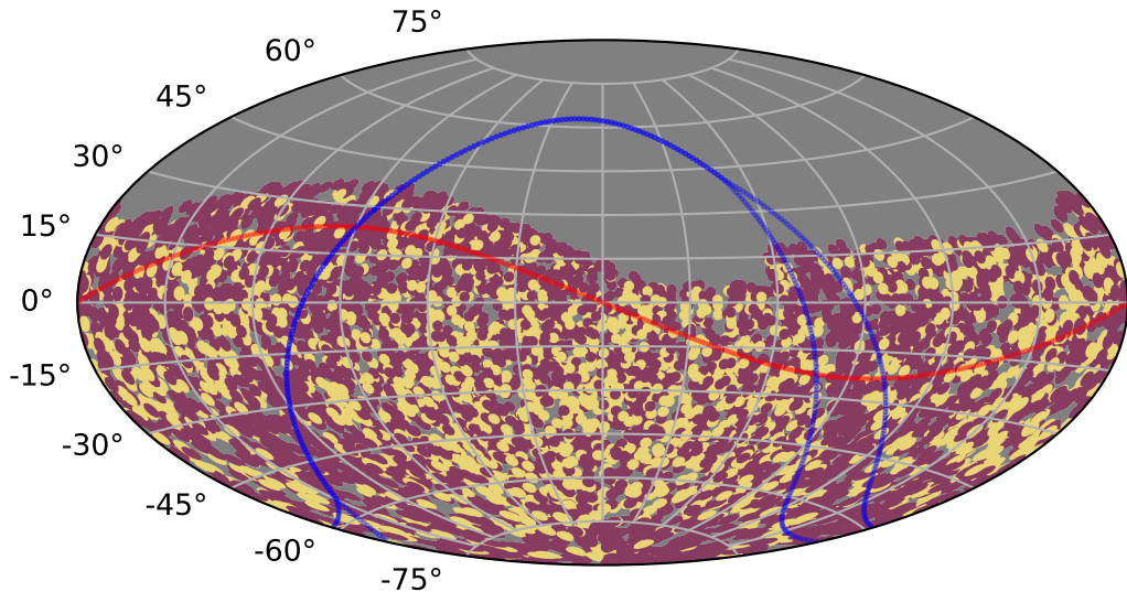
weather_cloudso4v3.5_10yrs : TDEsPopMetric_prepeak
