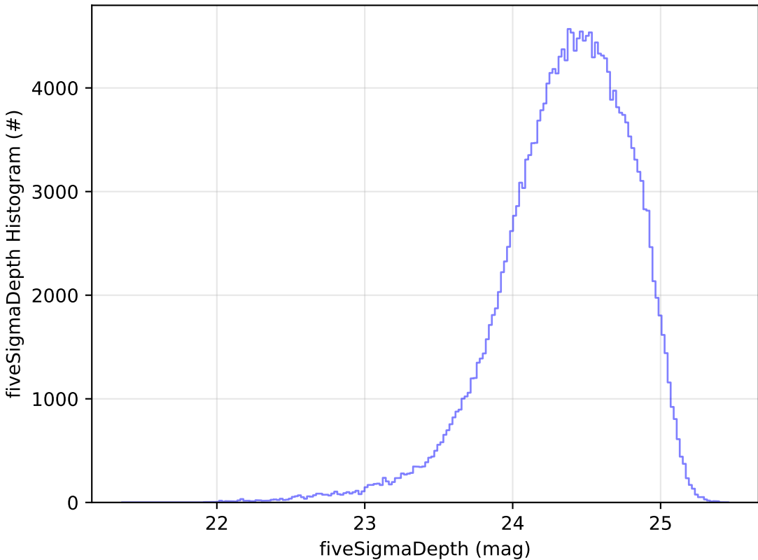
weather_cloudso4v3.5_10yrs g: fiveSigmaDepth Histogram
