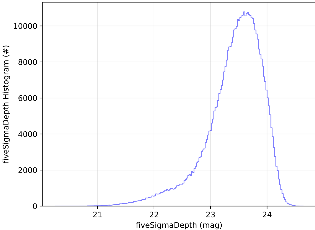
weather_cloudso4v3.5_10yrs i: fiveSigmaDepth Histogram
