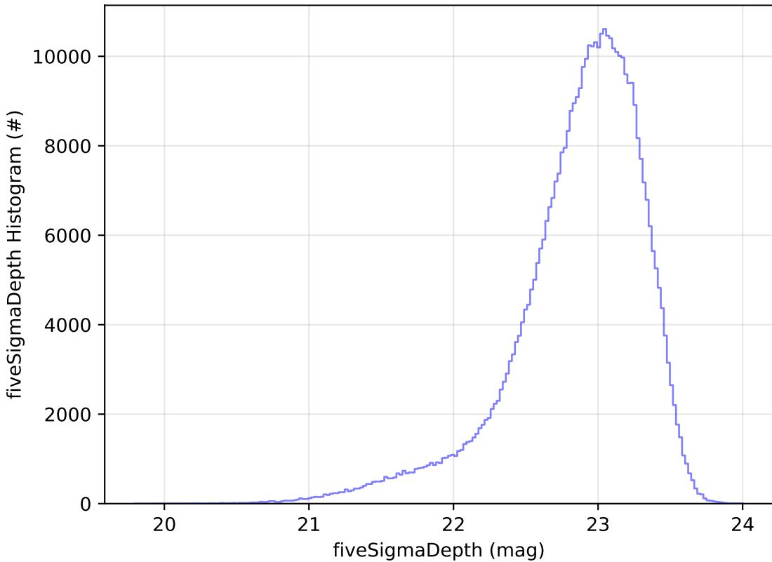
weather_cloudso4v3.5_10yrs z: fiveSigmaDepth Histogram
