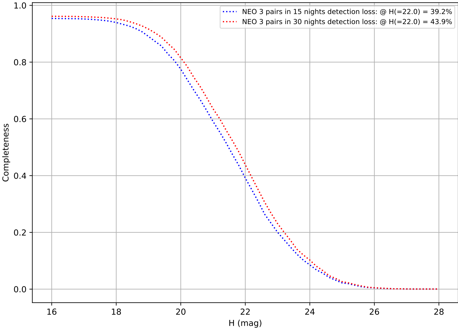
weather_cloudso4v3.5_10yrs: DifferentialCompleteness
