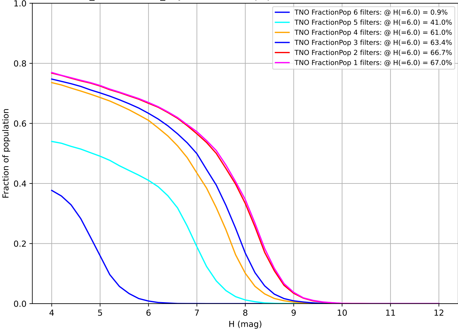
weather_cloudso4v3.5_10yrs: Fraction of population with colors in X filters TNO
