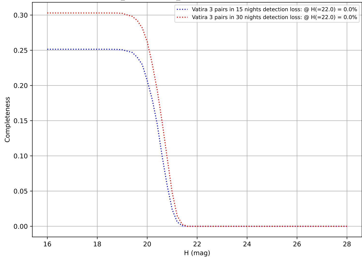
weather_cloudso4v3.5_10yrs: DifferentialCompleteness
