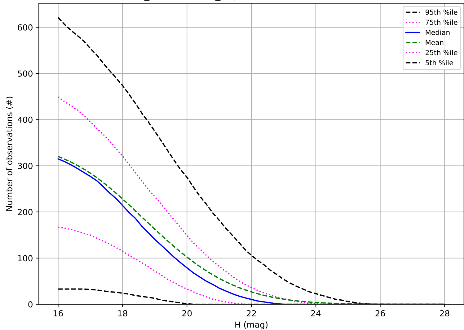
weather_cloudso4v3.5_10yrs: Number of observations NEO
