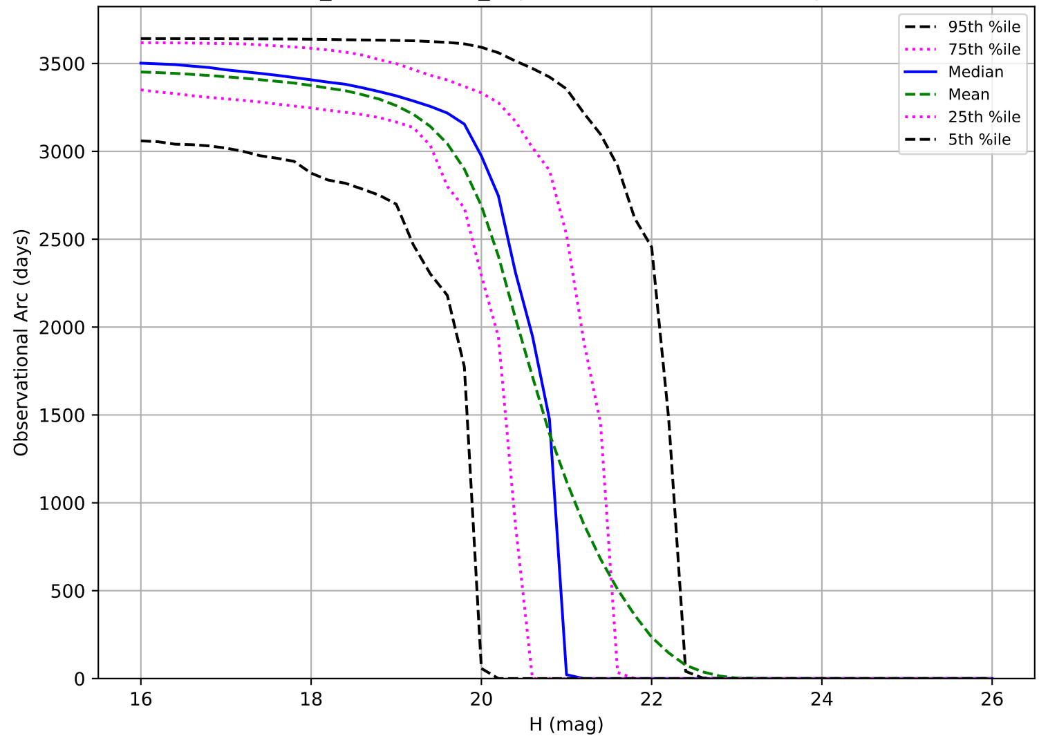
weather_cloudso4v3.5_10yrs: Observational Arc Length MBA
