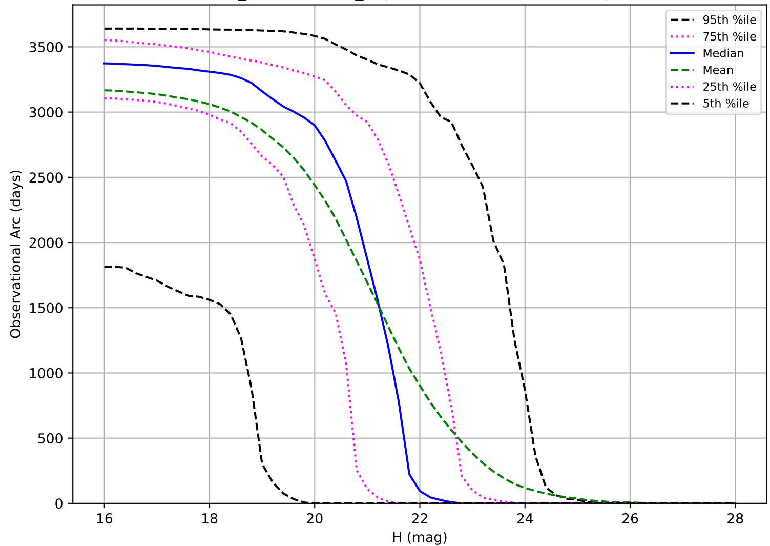
weather_cloudso4v3.5_10yrs: Observational Arc Length NEO
