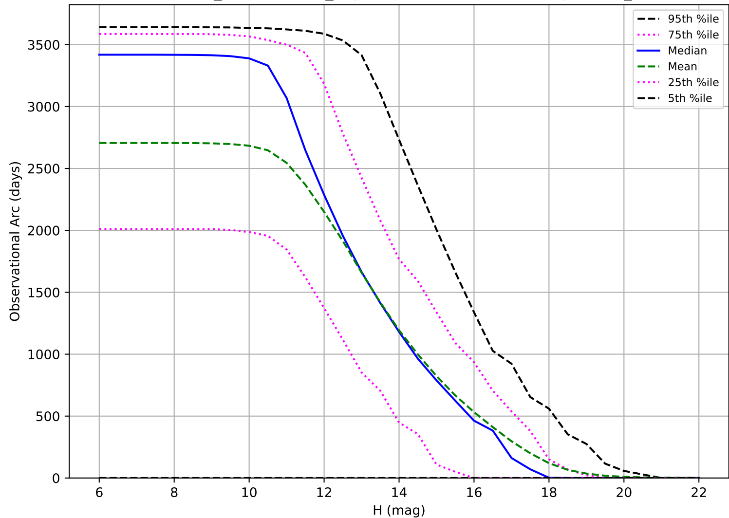
weather_cloudso4v3.5_10yrs: Observational Arc Length OCC_r5
