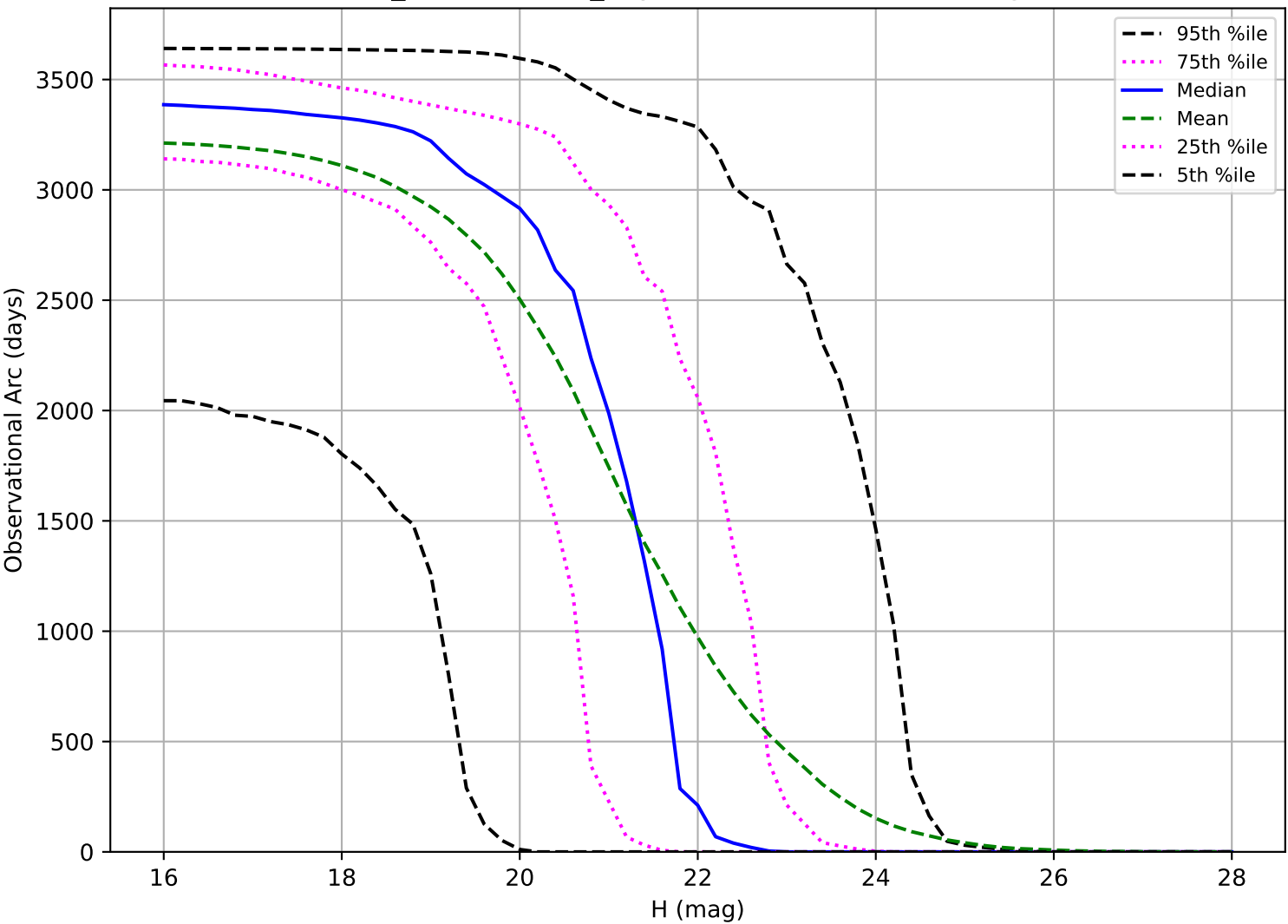
weather_cloudso4v3.5_10yrs: Observational Arc Length PHA
