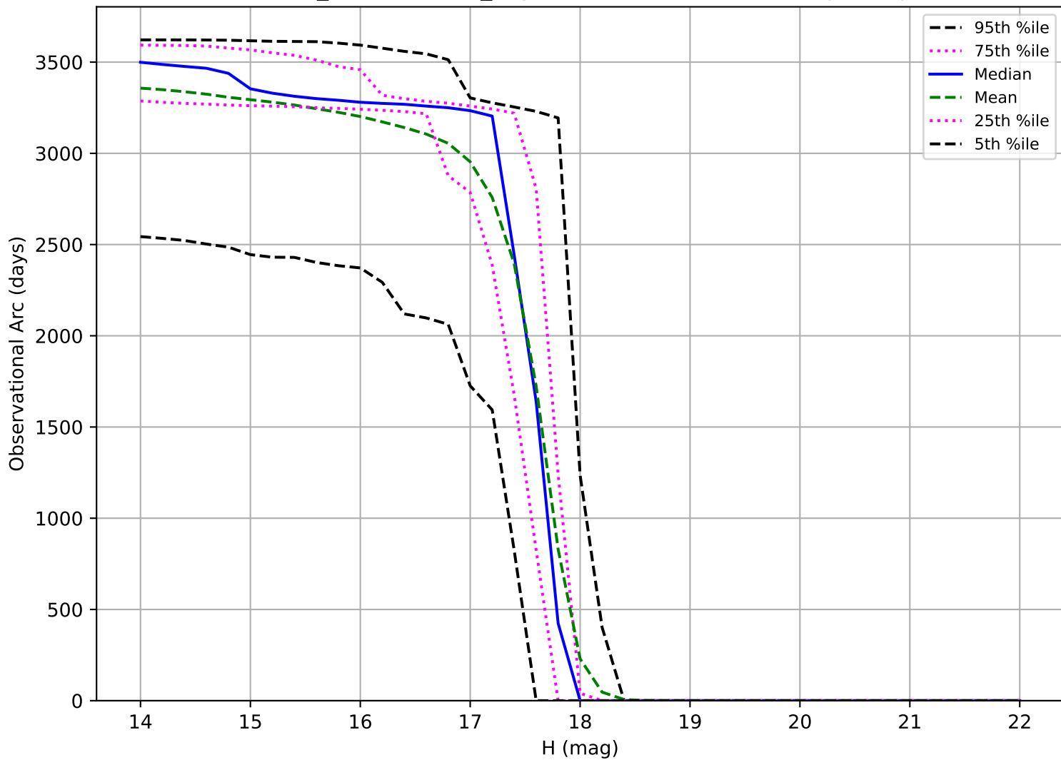
weather_cloudso4v3.5_10yrs: Observational Arc Length Trojan
