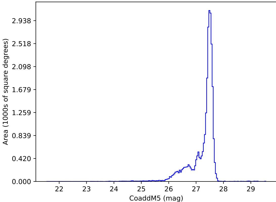
weather_cloudso6v3.5_10yrs : CoaddM5
