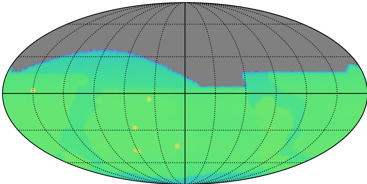
weather_cloudso6v3.5_10yrs : CoaddM5
