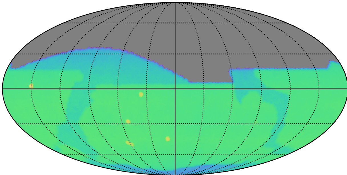
weather_cloudso6v3.5_10yrs r: CoaddM5
