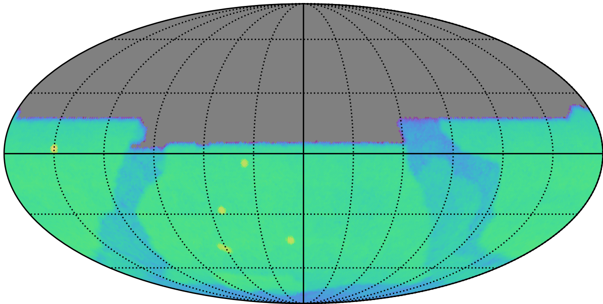
weather_cloudso6v3.5_10yrs u: CoaddM5
