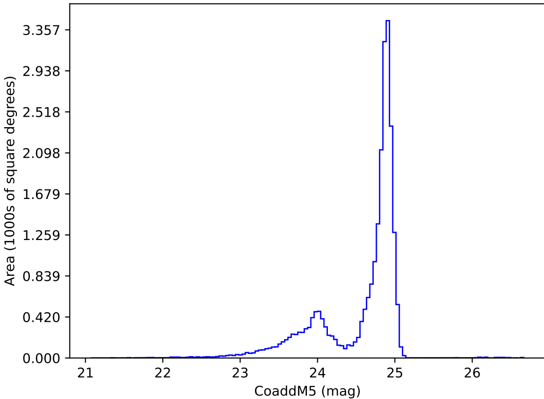
weather_cloudso6v3.5_10yrs y: CoaddM5
