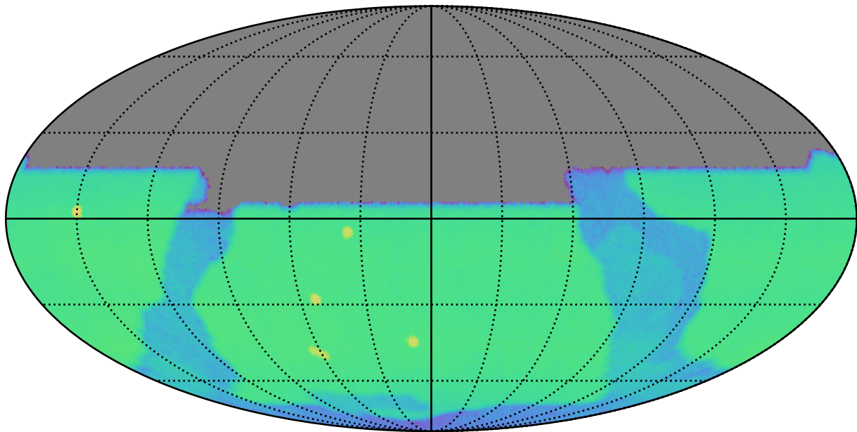
weather_cloudso6v3.5_10yrs y: CoaddM5
