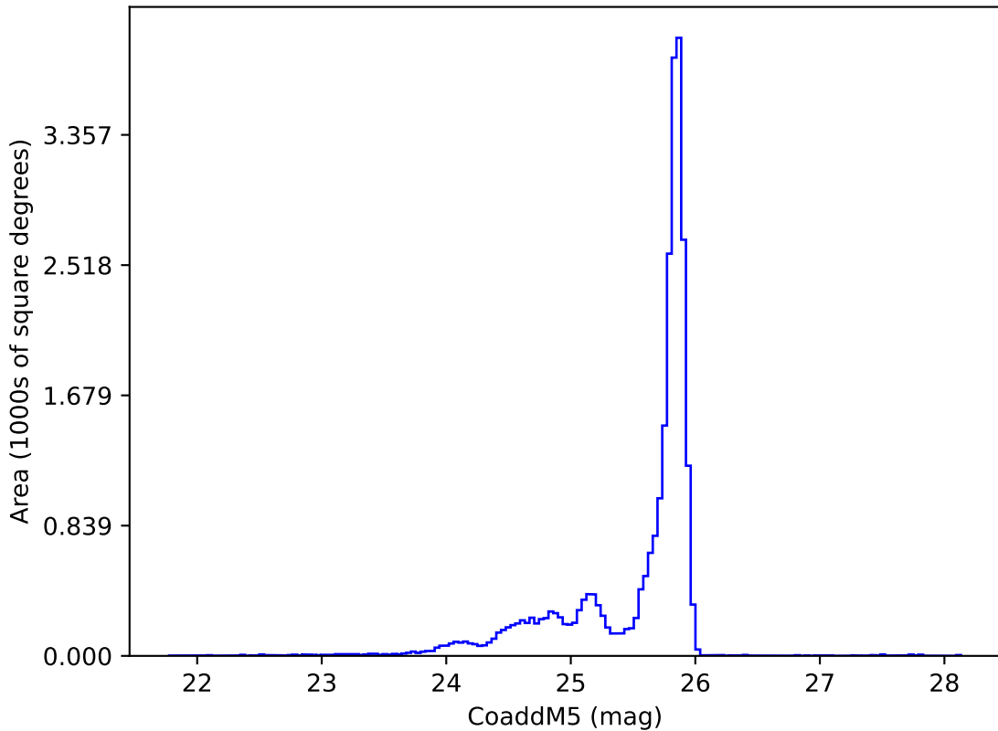
weather_cloudso6v3.5_10yrs z: CoaddM5
