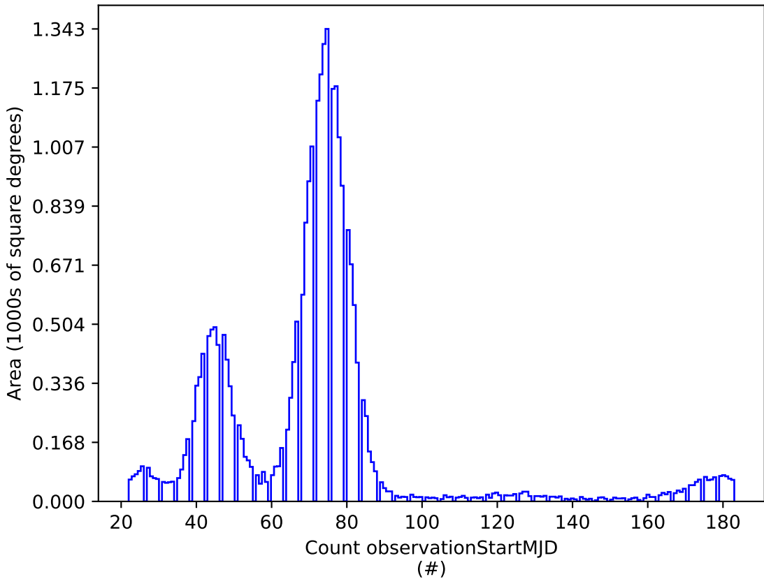
weather_cloudso6v3.5_10yrs g: Count observationStartMJD
