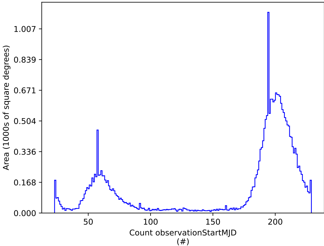
weather_cloudso6v3.5_10yrs i: Count observationStartMJD
