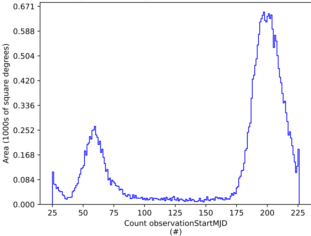
weather_cloudso6v3.5_10yrs r: Count observationStartMJD
