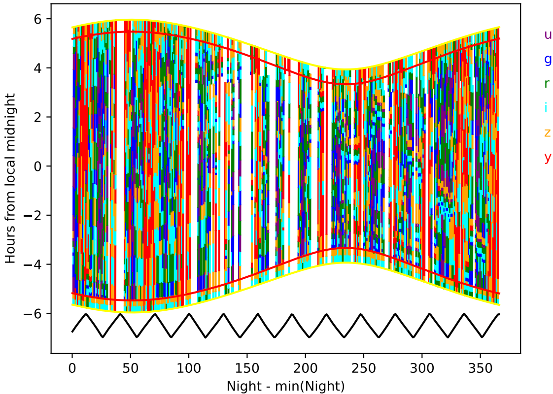
weather_cloudso6v3.5_10yrs year 0-1: Hourglass
