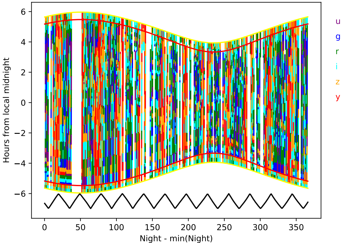
weather_cloudso6v3.5_10yrs year 2-3: Hourglass
