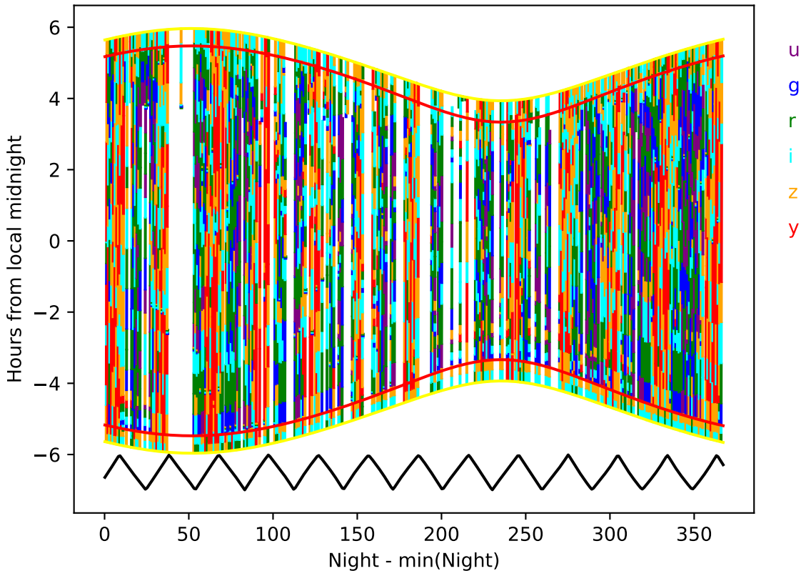
weather_cloudso6v3.5_10yrs year 3-4: Hourglass
