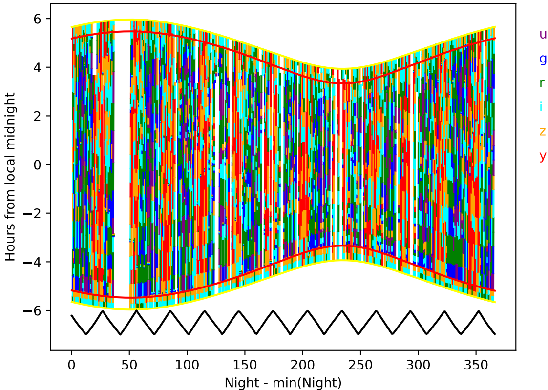
weather_cloudso6v3.5_10yrs year 4-5: Hourglass
