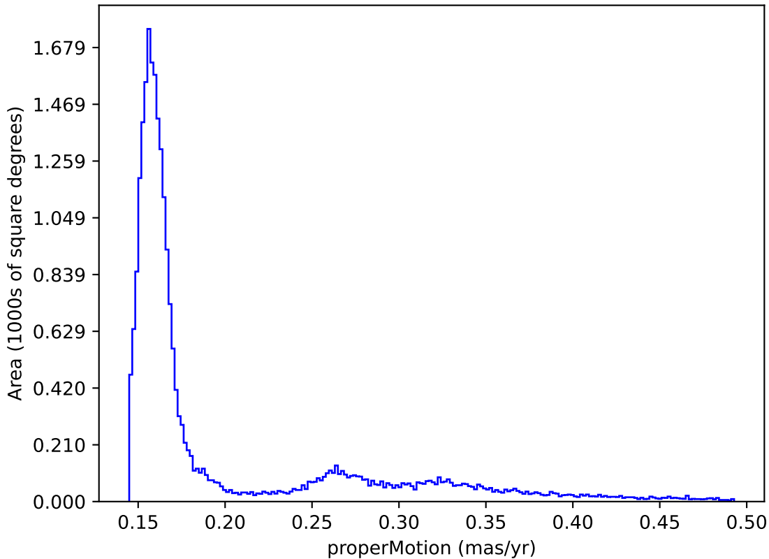
weather_cloudso6v3.5_10yrs : properMotion
