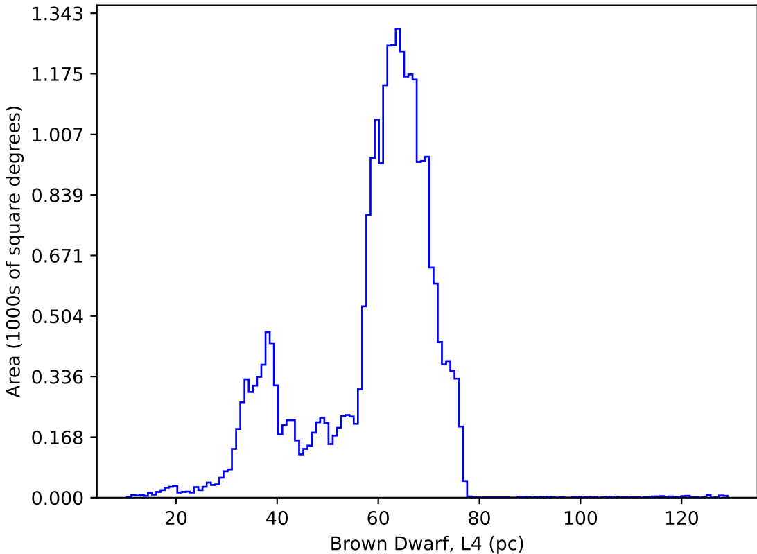
weather_cloudso6v3.5_10yrs : Brown Dwarf, L4
