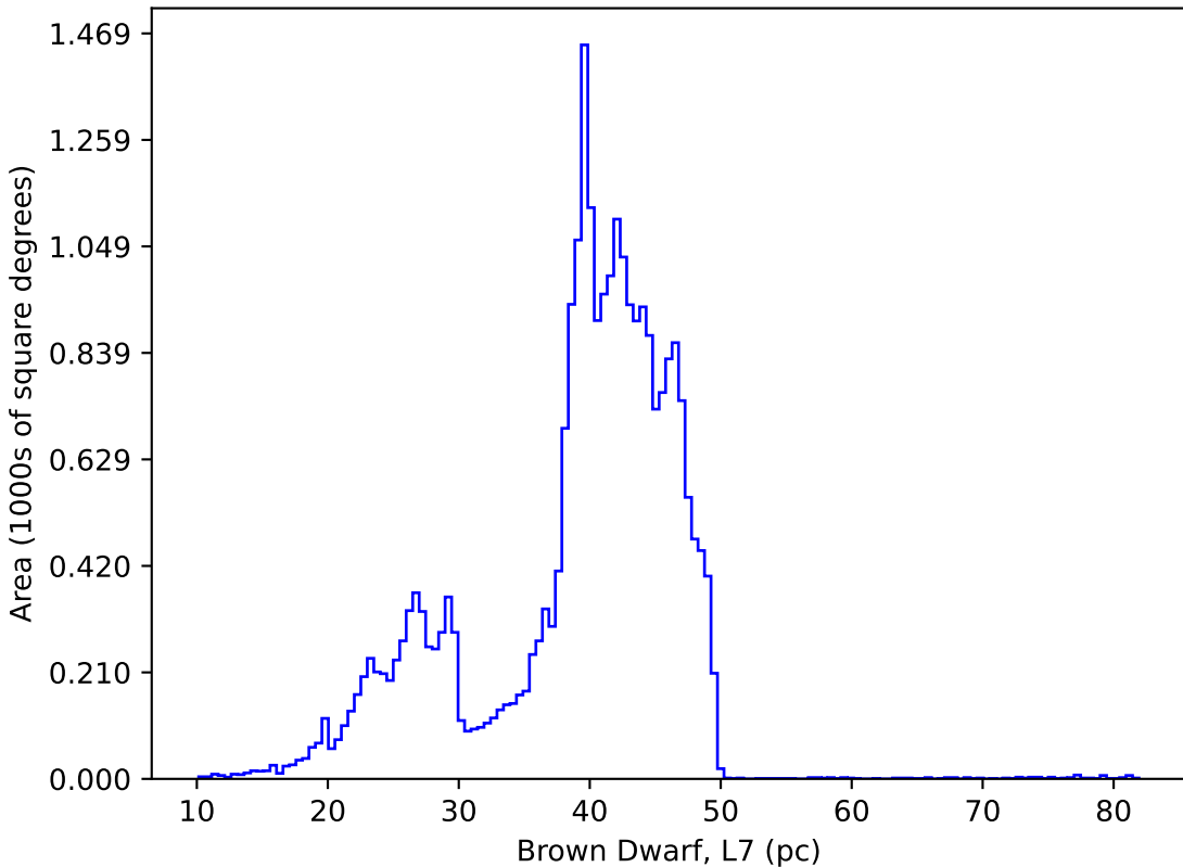
weather_cloudso6v3.5_10yrs : Brown Dwarf, L7
