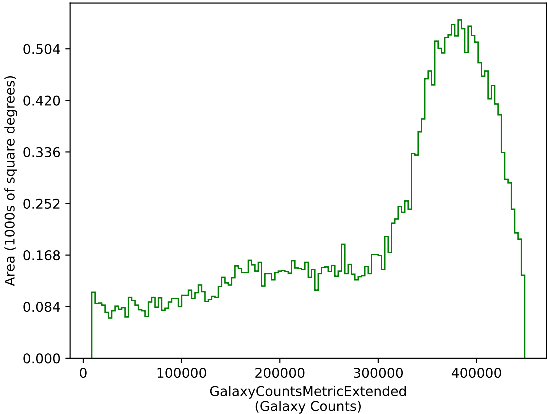
weather_cloudso6v3.5_10yrs g: GalaxyCountsMetricExtended
