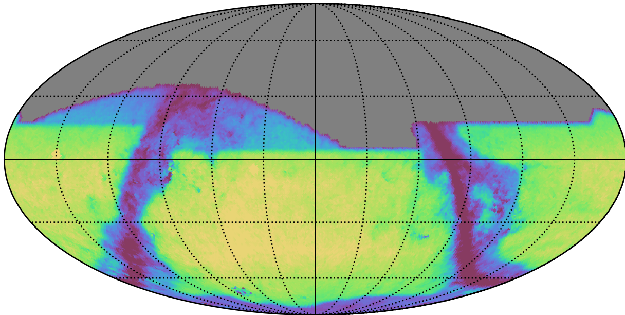
weather_cloudso6v3.5_10yrs i: GalaxyCountsMetricExtended
