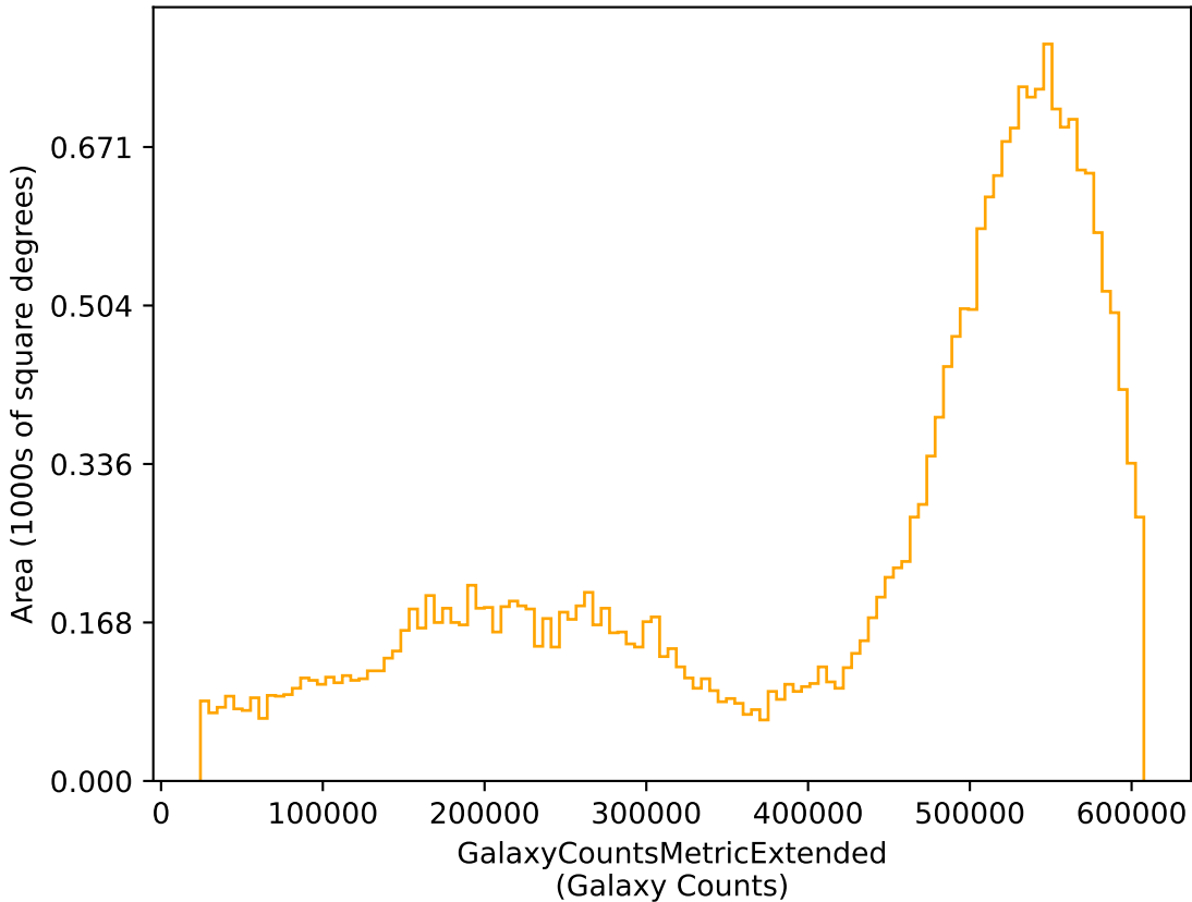
weather_cloudso6v3.5_10yrs r: GalaxyCountsMetricExtended
